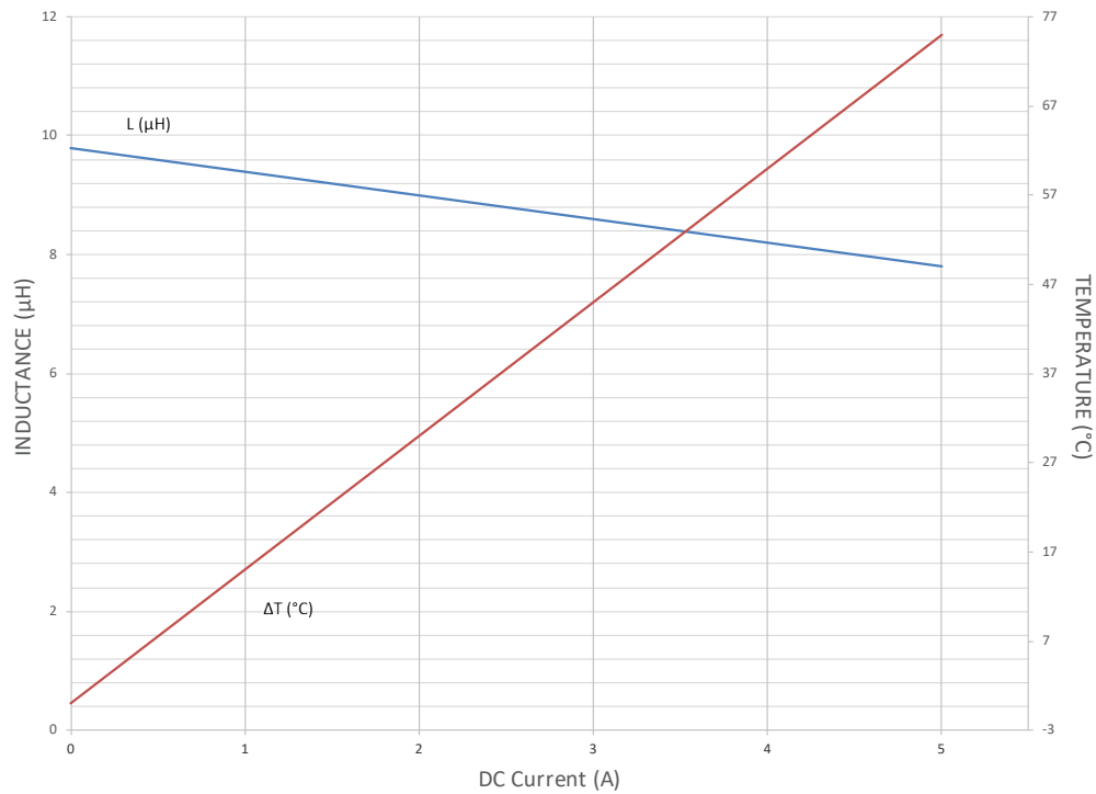
L&I Curve
