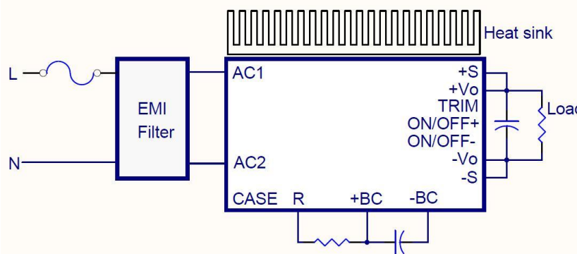
Simplified Application Circuit
