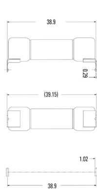
ZXPCB PCB Mount
