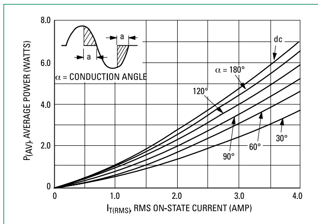
Figure 4. Power Dissipation
