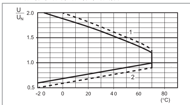
R 7S - DC coil operating range v ambient temperature - 7S.12/32 / 7S.23 / 7S.14/34 / 7S.16/36
