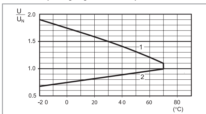
R 7S - DC coil operating range v ambient temperature - 7S.43/63
