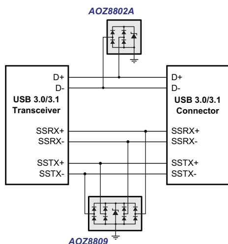
Figure 1. USB 3.0/3.1 Ports
