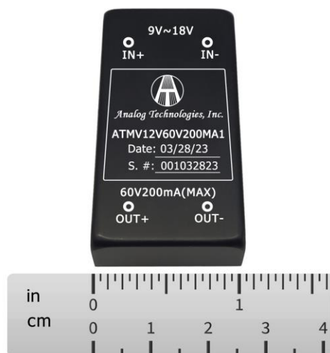
Figure 1. Top View
