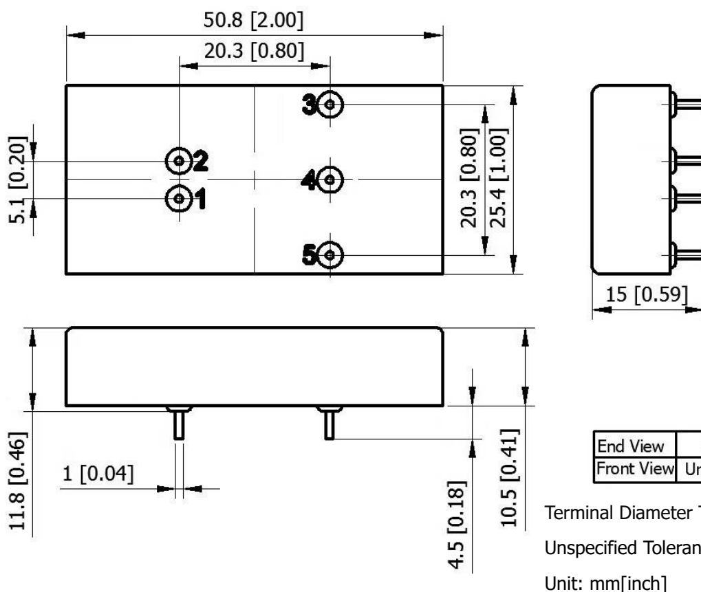
Figure 6. Outline Dimensions
