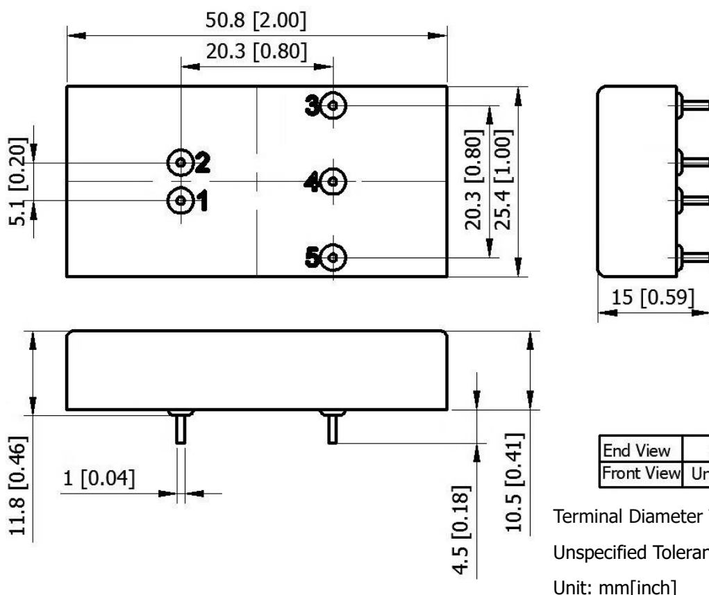
Figure 6. Outline Dimensions
