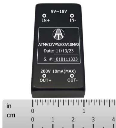
Figure 1. Top View of ATMV12VPN200V10MA2
