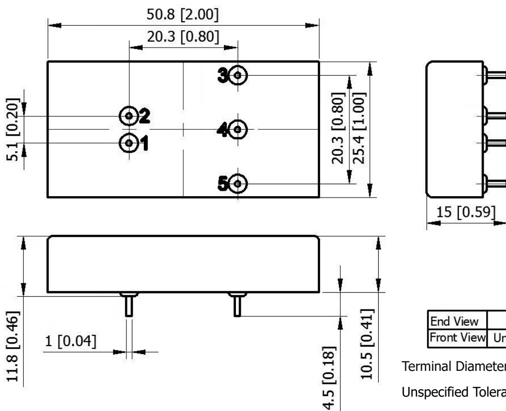
Figure 6. Outline Dimensions
