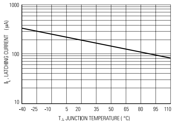
Figure 5. Typical Latching Current vs. Junction Temp
