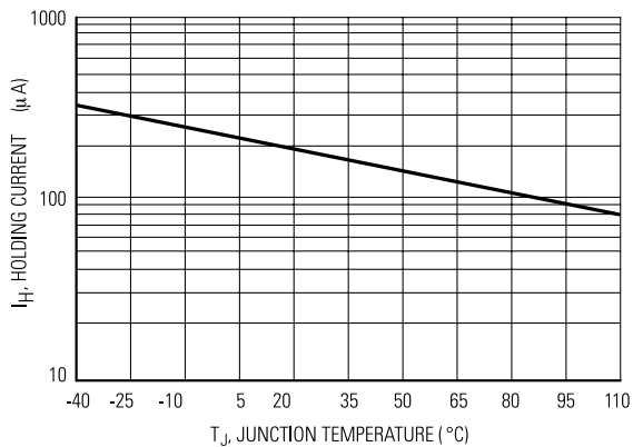
Figure 4. Typical Holding Current vs. Junction Temp
