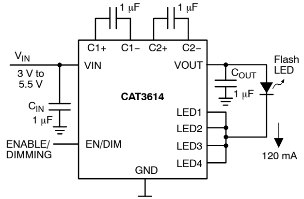
Figure 29. Single Flash LED Application
