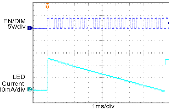
Figure 14. Dimming Levels
