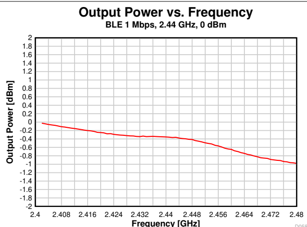
Figure 8-29. Output Power vs. Frequency (BLE 1 Mbps, 2.44 GHz)
