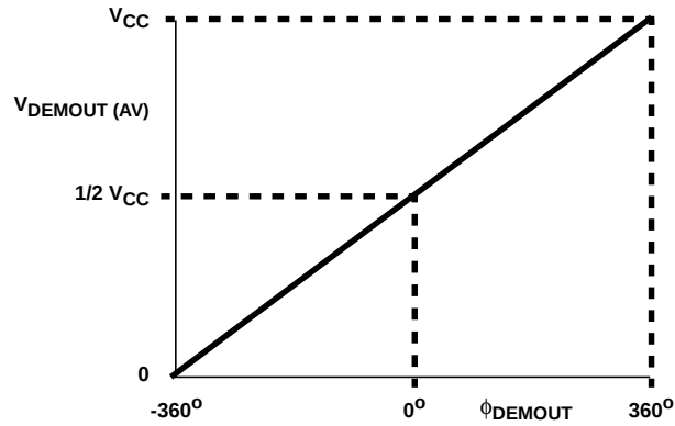
FIGURE 4. PHASE COMPARATOR 2: AVERAGE OUTPUT VOLTAGE vs INPUT PHASE DIFFERENCE: V_{\text{DEMOUT}} = V_{\text{PC2OUT}} = (V_{\text{CC}}/\pi) (\phi_{\text{SIGIN}} - \phi_{\text{COM-}}) \phi_{\text{DEMOUT}} = (\phi_{\text{SIGIN}} - \phi_{\text{COMPIN}})
