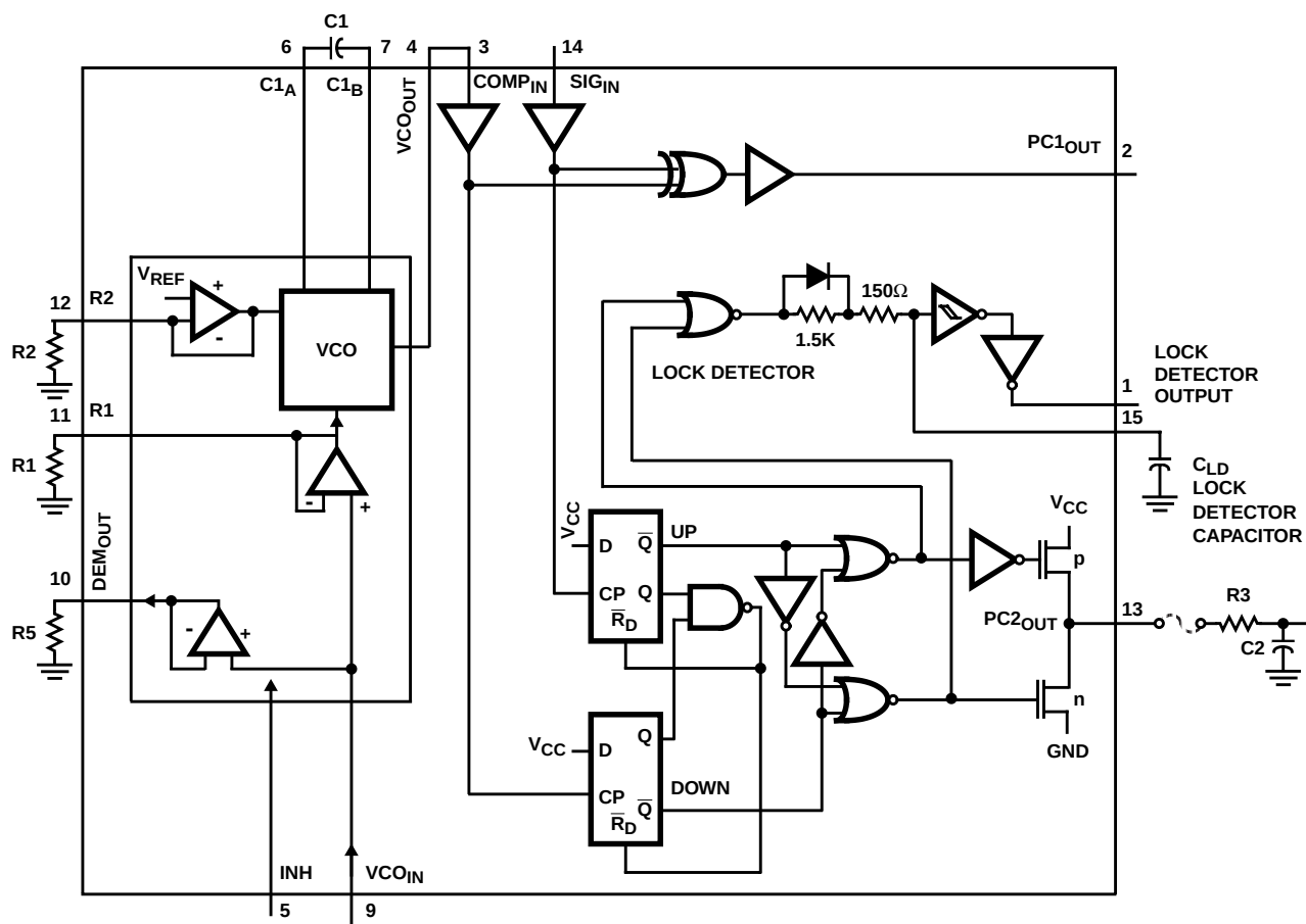
FIGURE 1. LOGIC DIAGRAM
