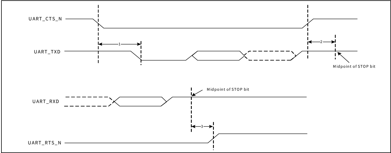
Figure 8 UART timing
