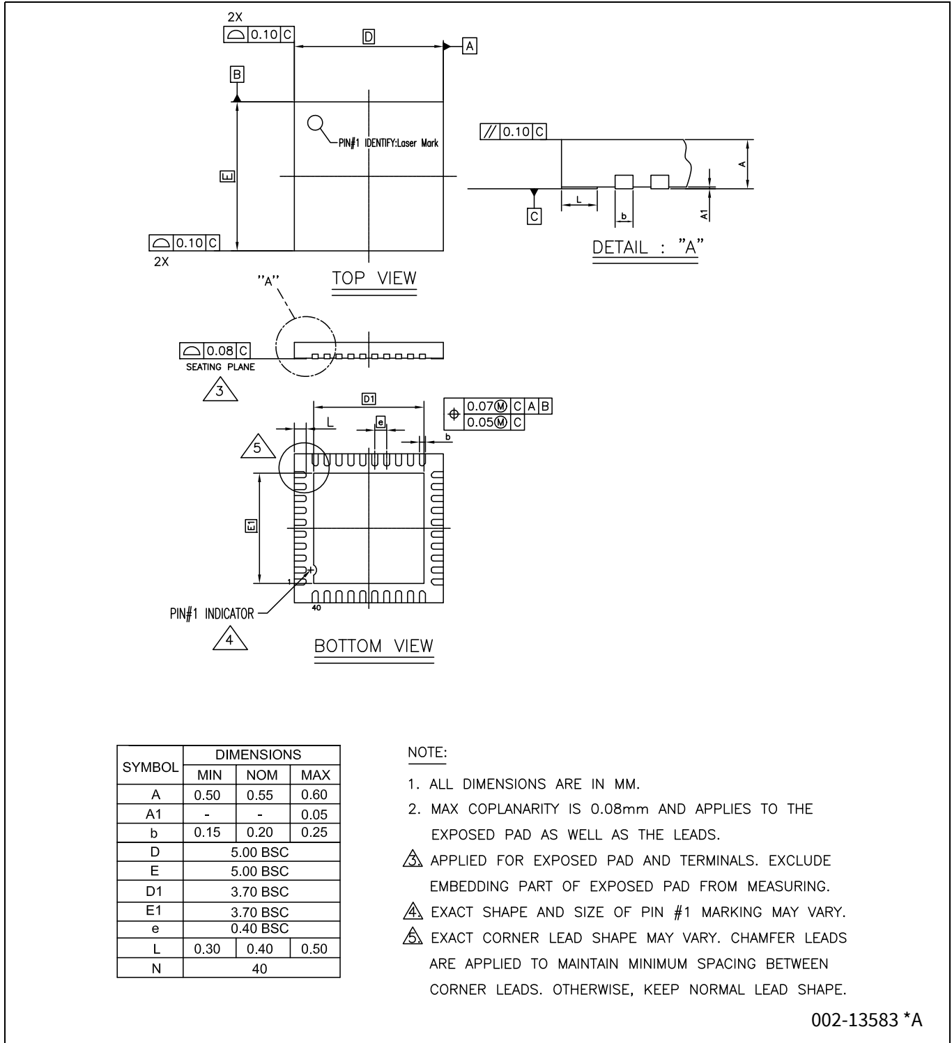
Figure 14 CYW20719 5.0 mm x 5.0 mm 40-pin QFN package (PG-VQFN-40)
