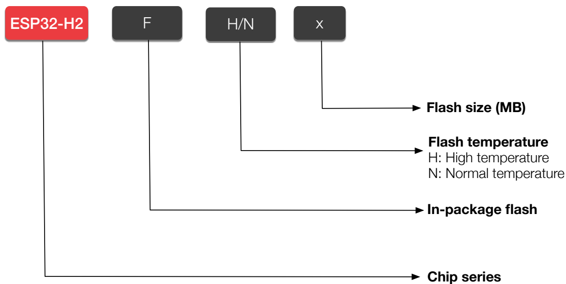
Figure 1-1. ESP32-H2 Series Nomenclature
