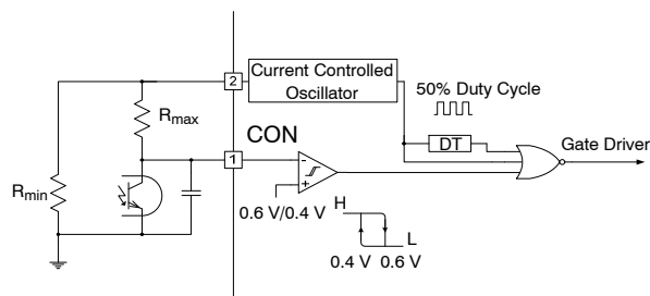
Figure 42. Pulse-Skipping Circuit
