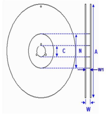
Fig. 9.3 The dimension of reel
