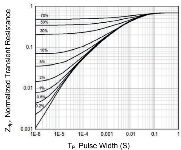
Figure 10. Transient Thermal Impedance vs. T_P
