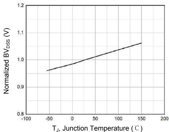
Figure 4. Normalized BV_{DS} Vs. Junction Temperature
