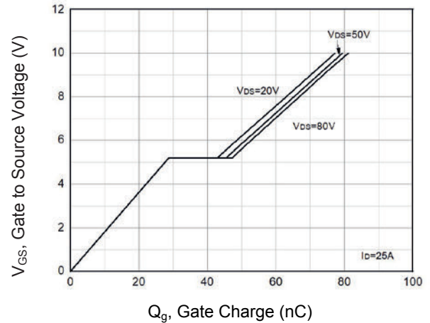
Figure 8. Gate Charge.
