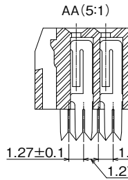
■A-A cross section
