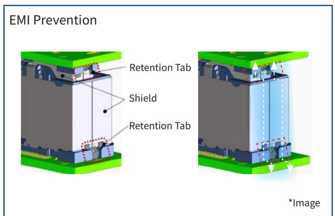
Shield Grounding Design
