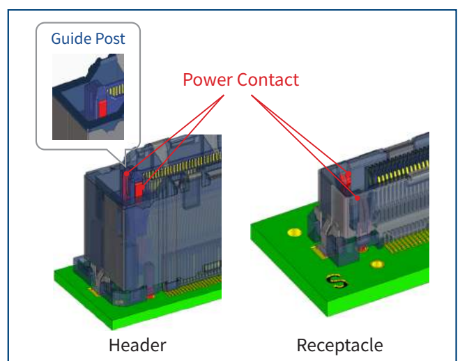
Hybrid Power & Signal Design with Large Guide Posts on Both Ends
