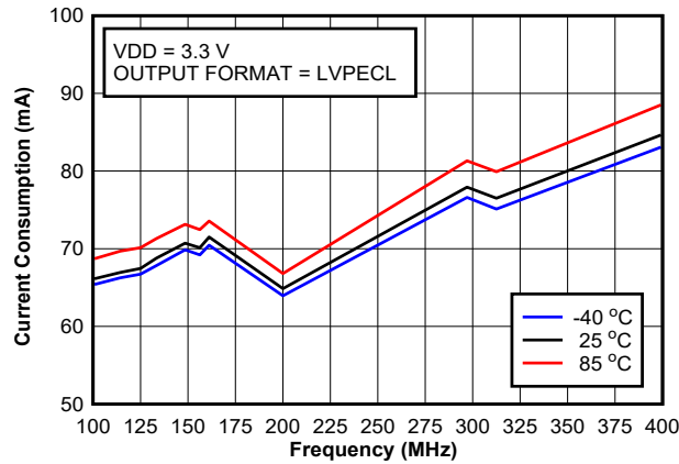
Figure 6-11. Current Consumption vs Frequency (LVPECL, 3.3V)
