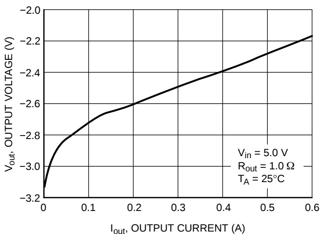
Figure 47. Current Boosted Load Regulation, Output Voltage vs. Output Current MAX829
