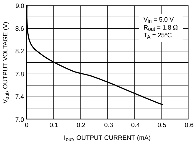
Figure 50. Positive Doubler with Current Boosted Load Regulation, Output Voltage vs. Output Current, MAX829
