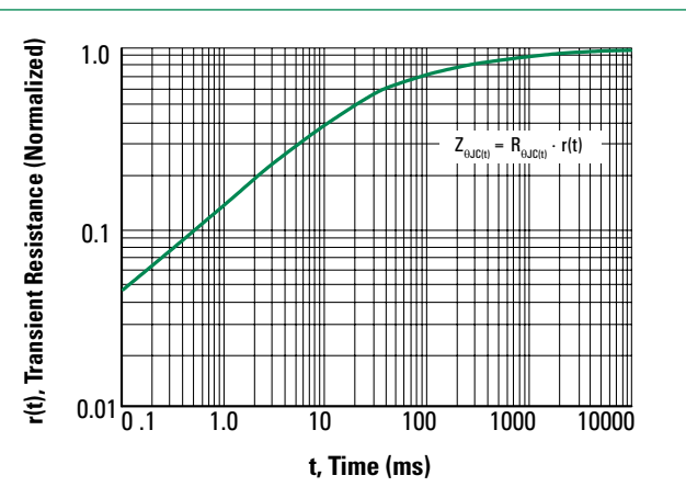
Figure 4. Transient Thermal Response
