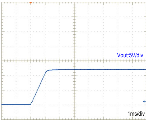
Figure 14. Vout Start-up
