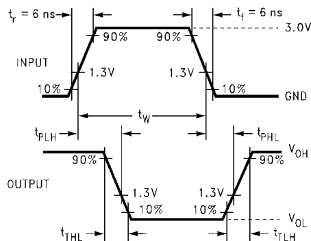
Figure 6. AC Waveforms
