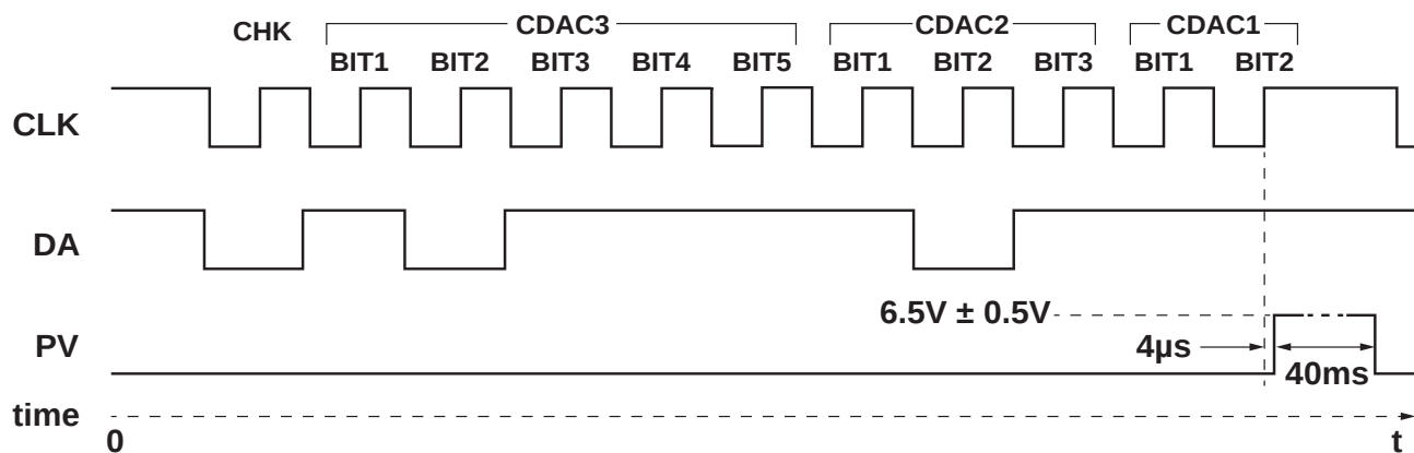
Figure 5: All-Bits Programming Sequence
