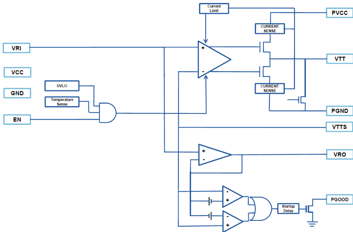
Figure 2. Block Diagram
