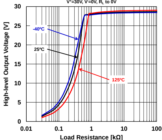
High-level Output Voltage vs. Load Resistance
