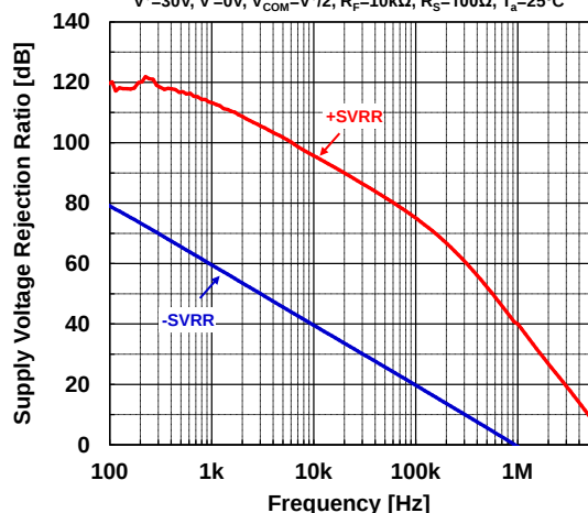
Supply Voltage Rejection Ratio vs. Frequency
