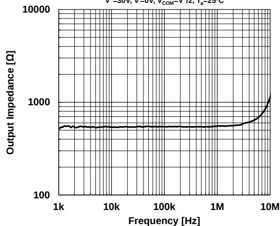
Output Impedance vs. Frequency
