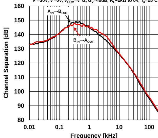
Channel Separation vs. Frequency (NJM2904B)
