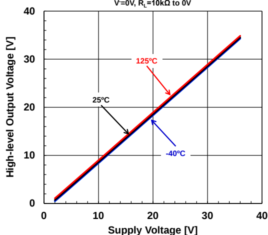
High-level Output Voltage vs. Supply Voltage
