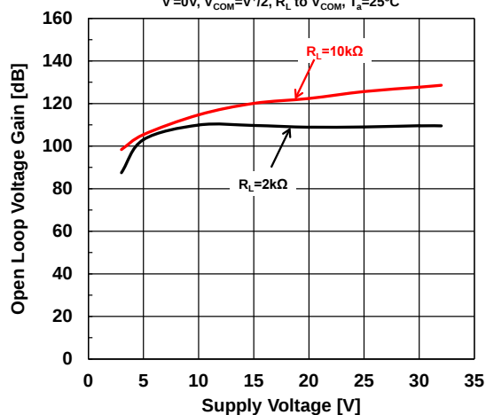
Open Loop Voltage Gain vs. Supply Voltage
