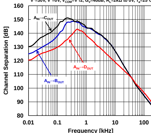
Channel Separation vs. Frequency (NJM2902B)
