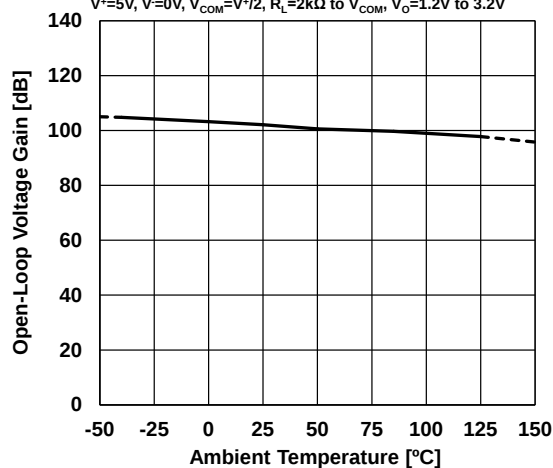
Open-Loop Voltage Gain vs. Temperature
