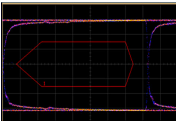
Figure 13. USB 1.1 Full Speed Eye Diagram
