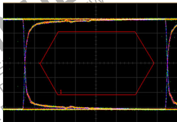
Figure 14. USB 1.0 Low Speed Eye Diagram
