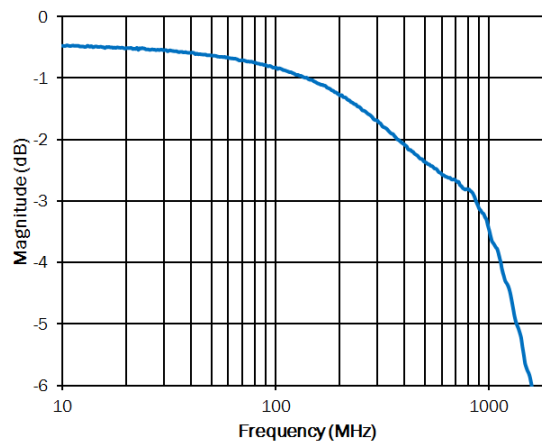
Figure 16. Data Switch Differential Insertion Loss
