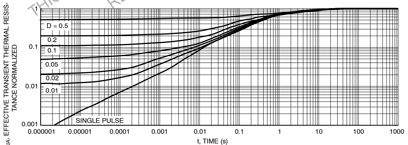
Figure 11. Thermal Response
