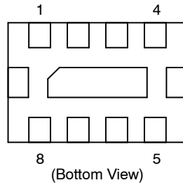
Figure 3. Pin Diagram
