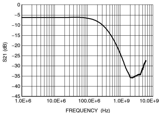
Figure 2. Typical Insertion Loss Characteristic
