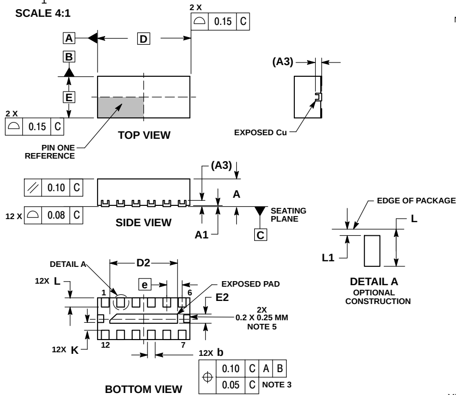
DFN12 3.0x1.35, 0.5P CASE 506AD ISSUE J
