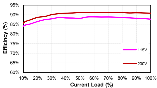
PDF700S560 (Eff Vs Io)
