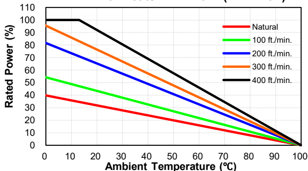
PDF700S240/280/480/560 Derating Curve with Heatsink M-B012 (Vin=115V)
