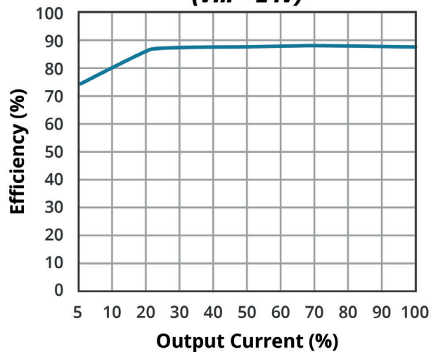
EFFICIENCY VS OUTPUT LOAD PDQE20-Q24-D5-U (Vin = 24V)
