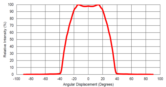
Radiation Pattern for 60 degree
