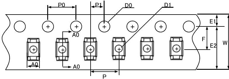
Component Orientation in Tape
