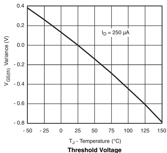
Threshold Voltage
