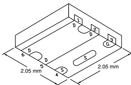
PowerPAK SC-70-6L-Single
