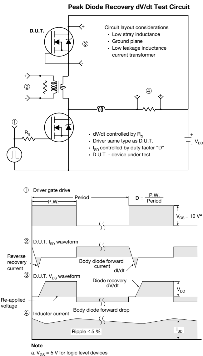
Fig. 20 - For N-Channel
