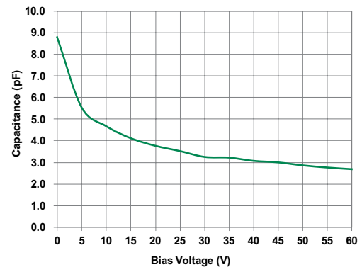
Capacitance vs. Reverse Bias
