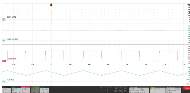
Figure 21. Pulse Skipping Operation
