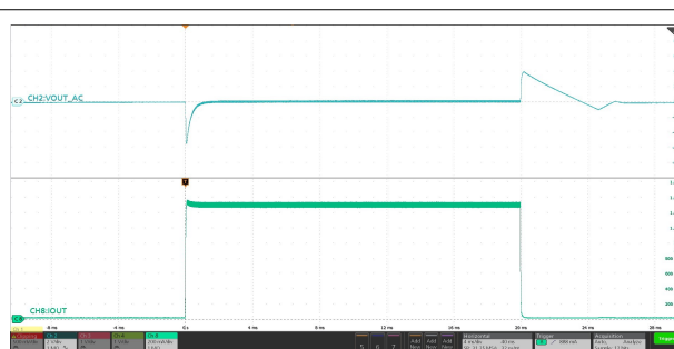
Figure 26. Load Transient Response
