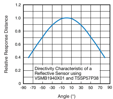
Fig. 10 - Angle Characteristic
