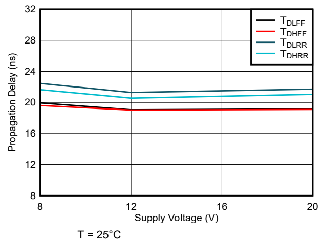
Figure 5-13. Propagation Delays vs Supply Voltage ( V_{DD} = V_{HB} )
