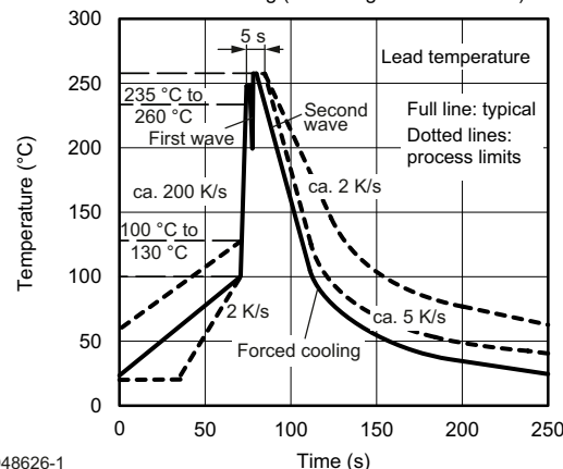
Fig. 27 - Double Wave Soldering of Opto Devices (all packages)
