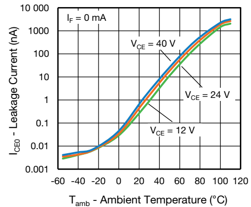
Fig. 8 - Collector Emitter Current vs. Ambient Temperature
