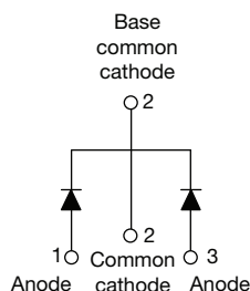
VS-15CTQ...-1-M3
