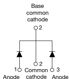
VS-15CTQ...S-M3
