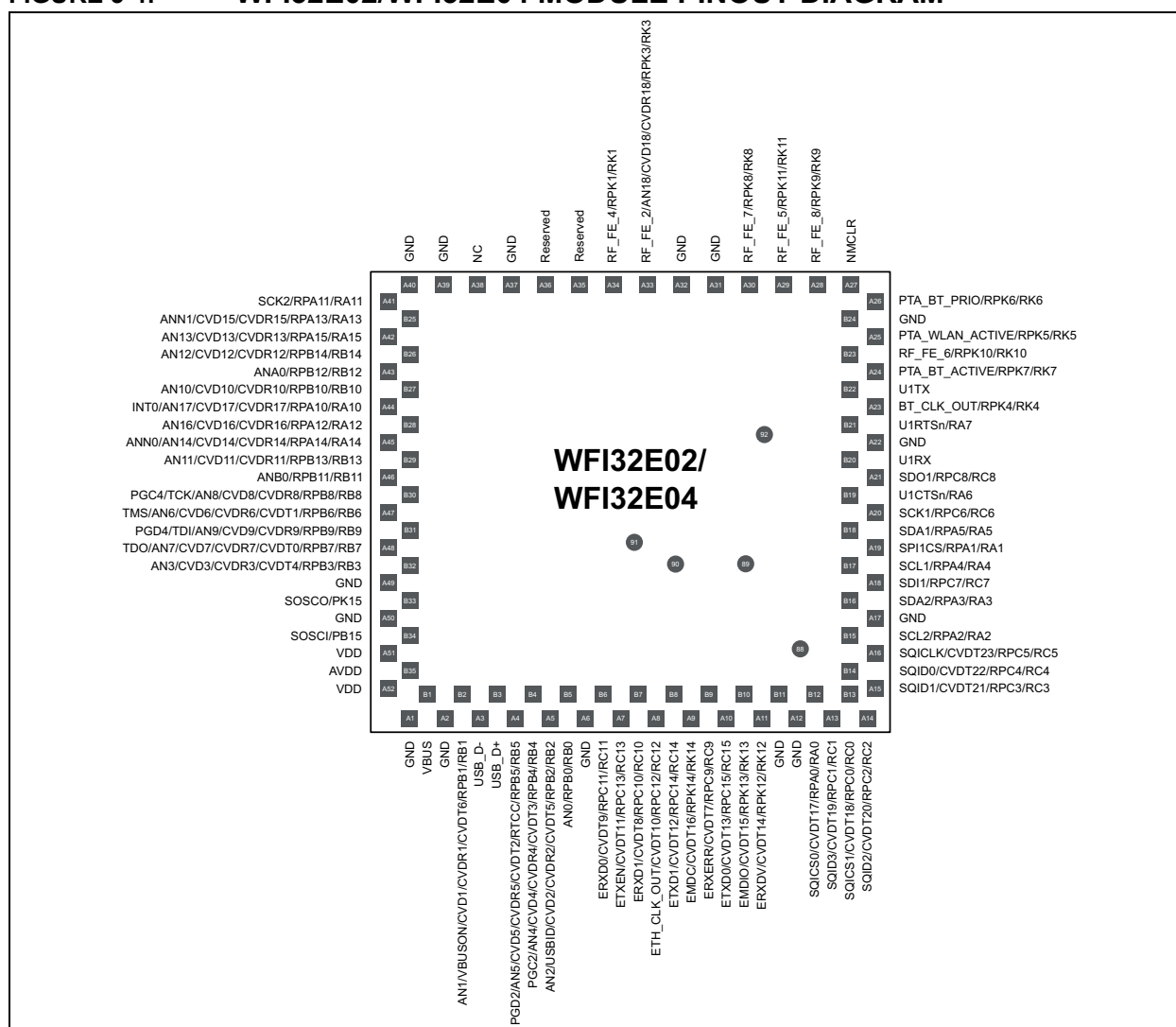
FIGURE 3-4: WFI32E02/WFI32E04 MODULE PINOUT DIAGRAM
