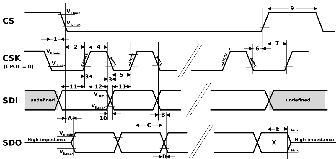
Figure 3: ZED-F9P-15B SPI specification mode 1: CPHA=0 SCK = 5.33 MHz
